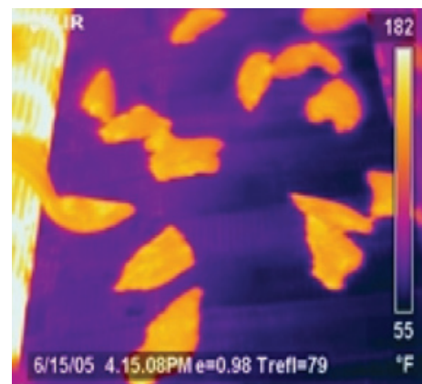
An IR temperature measurement and thermographic image are used to locate undercooked chicken tenders and stop the line so undercooked ones can be removed.
